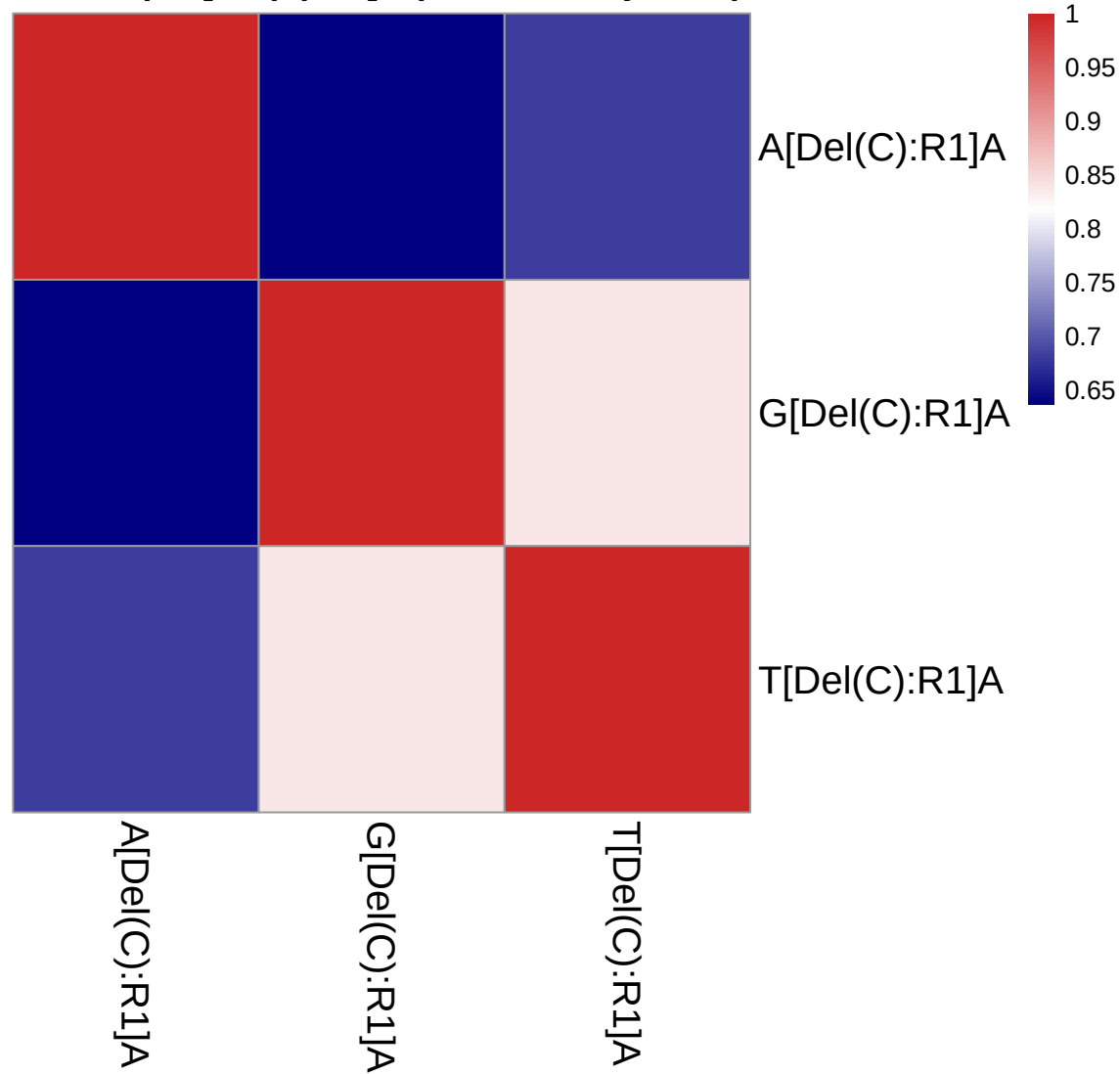
Heatmap – [Del(C):R1]A (Reordered by Base)
